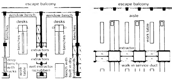
③ Laboratory equipment in main science lab (Bayer AG dye factory)
